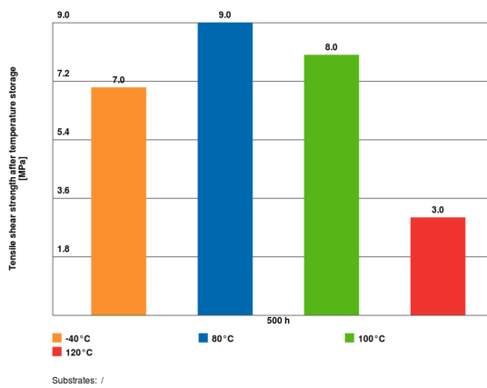
Tensile shear strength after temperature storage / based on DIN EN ISO 527
